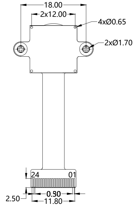
BOTTOM VIEW
